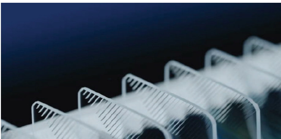
The “lines” visible in the finished waveguides are semi-transparent mirrors that convey the projector’s content to the eye precisely. Photo: SCHOTT
