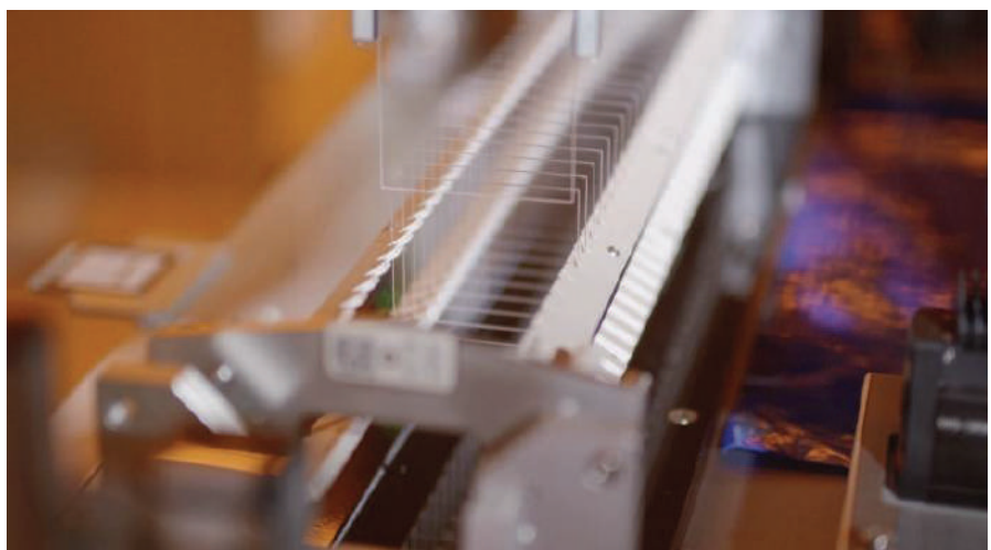
Waveguide manufacturing before shaping. A robot removes the glass fully automatically for downstream processing in a machine. Photo: SCHOTT
