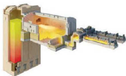
Oxyfuel Furnaces
