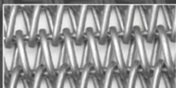
TYPE L.K.16 SPECIFICATION 36-22-12-12 (LEHR BELT)
