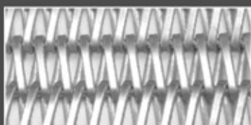
TYPE L.K.16 FLAT SPECIFICATION 36-22-3 X 1.75-12 (LEHR BELT)
